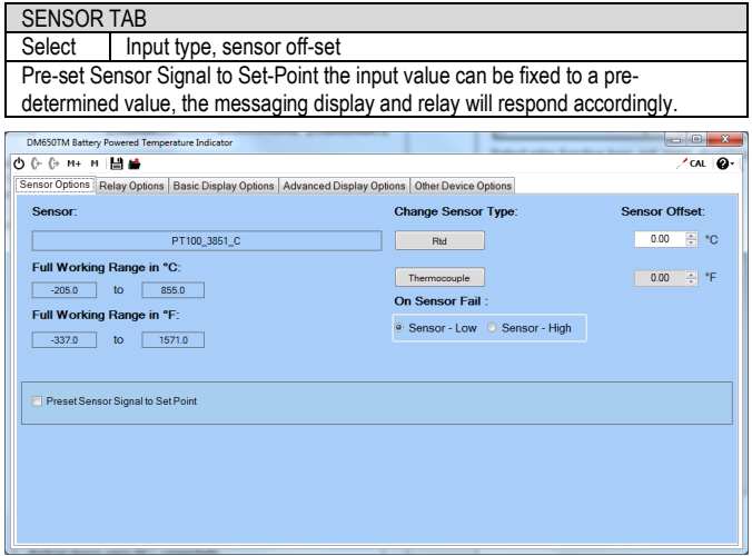
DM650TM configuration software (Sensor Options Tab).
